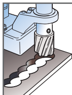
Overlapped cutting
